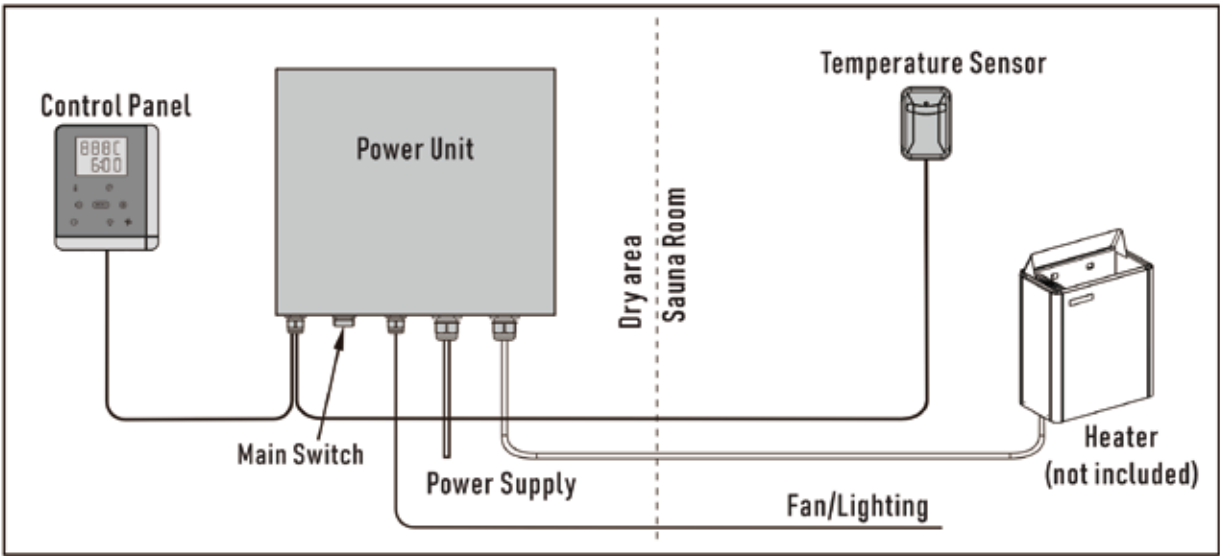
Controller Installation Diagram
