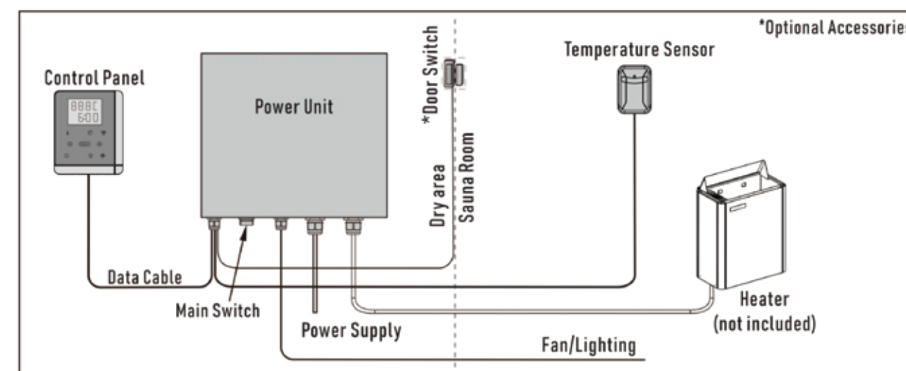
Controller Installation Diagram
